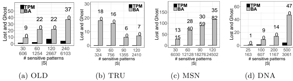
Fig. 4: Total number of \tau -lost and \tau -ghost patterns vs. number of sensitive patterns (and |\mathcal{S}| ). \frac{x}{y} on the top of each bar for BA denotes x \tau -lost and y \tau -ghost patterns.
